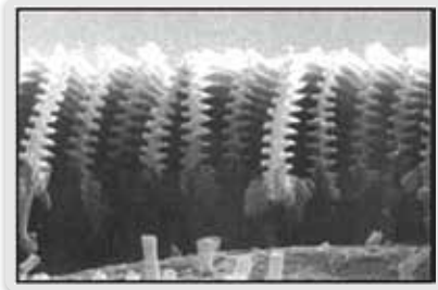
Figure 2. Nano-patterned phonic
